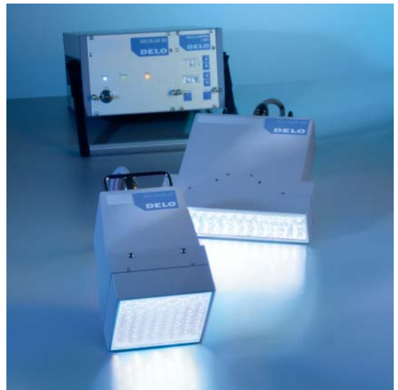
DELOLUX 20 / DELOLUX 202 LED area lamps, light exit area 101 x 101 mm 2 (DELOLUX 20) or 48.1 x 198.4 mm 2 (DELOLUX 202)
